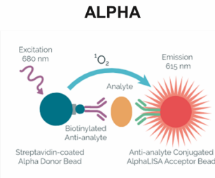
Amplified Luminescent Proximity Homogeneous Assay
