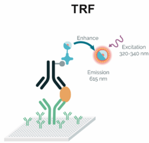
Time Resolved Fluorescence
