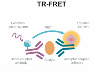
Time Resolved Fluorescence Resonance Energy Transfer
